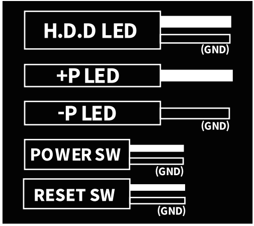
Conector Power/Reset/LED do Gabinete
