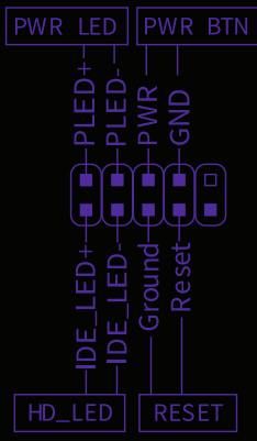
Motherboard Power/Reset/LED Connector
