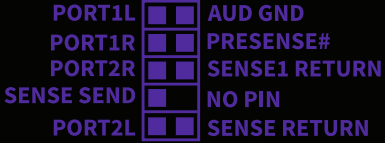
Motherboard HD Audio Connector
