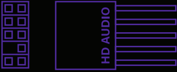
Case HD Audio Connector
