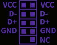
Motherboard USB 2.0 Connector
