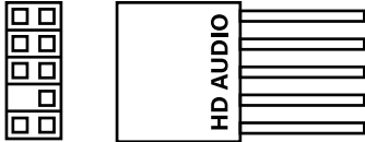
Case HD Audio Connector
