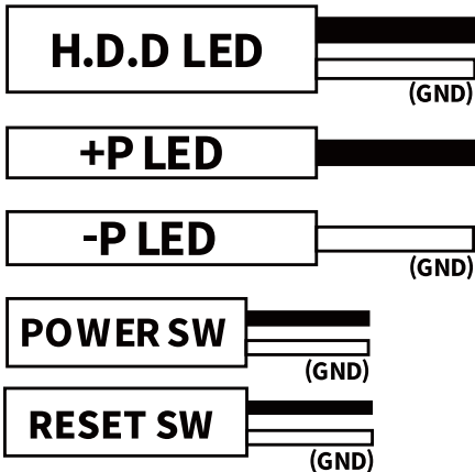
Case Power/Reset/LED Connector
