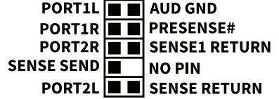
Motherboard HD Audio Connector
