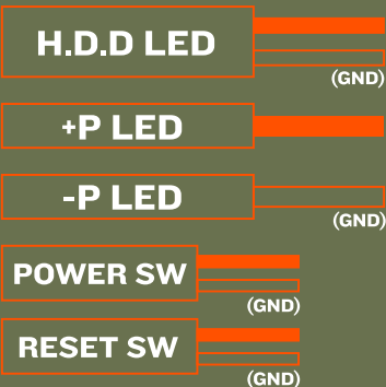
Conector Power/Reset/LED do Gabinete
